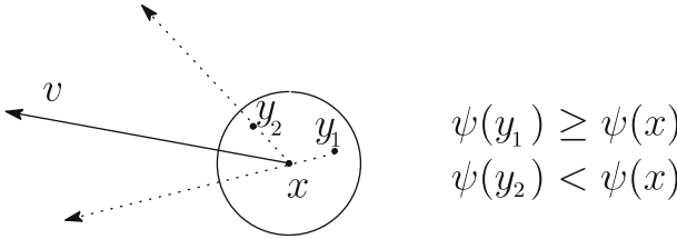
Figure 2. An ADD example in R^2 .
