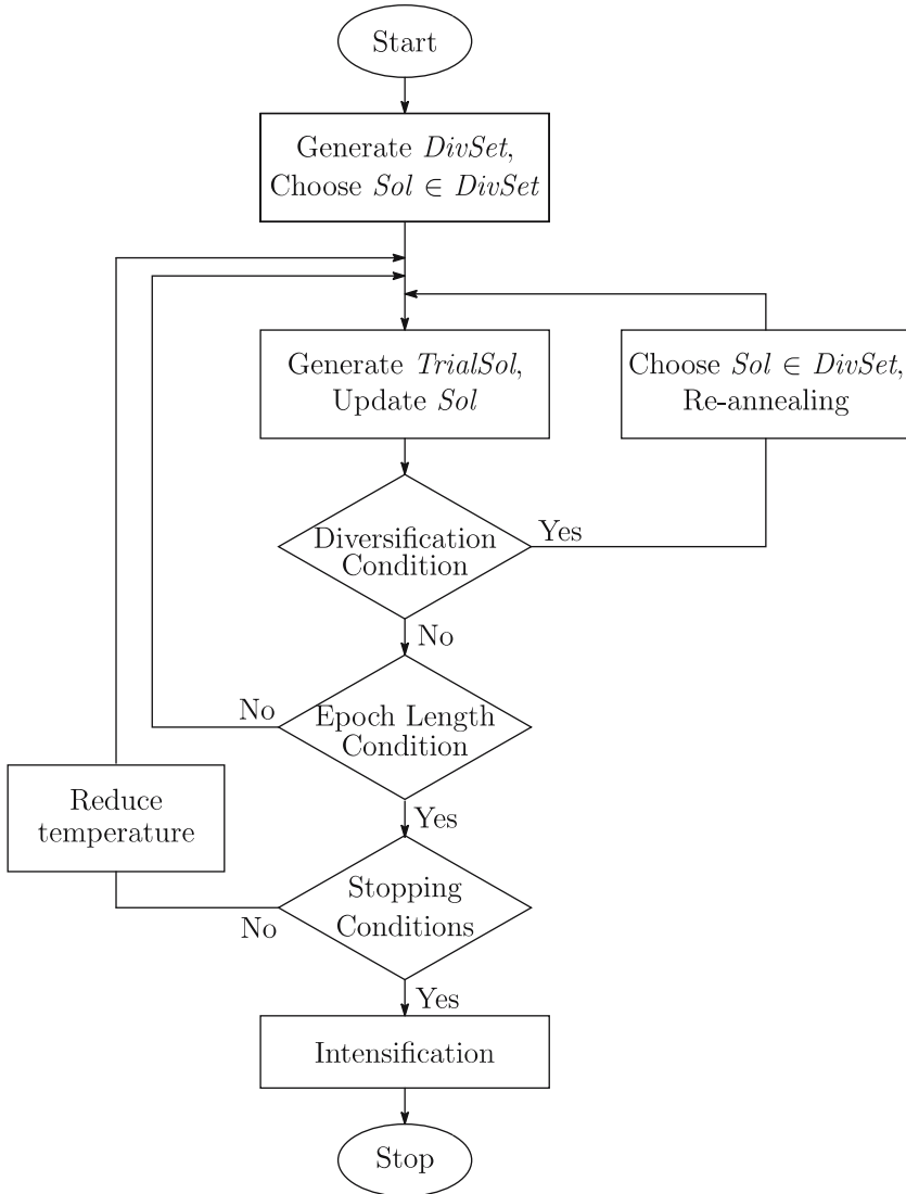
Figure 1. Outline of the FSA method.
