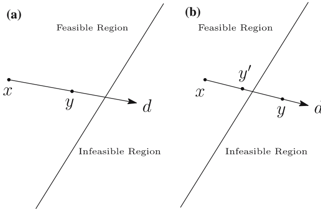
Figure 3. An example of generating trial solutions.
